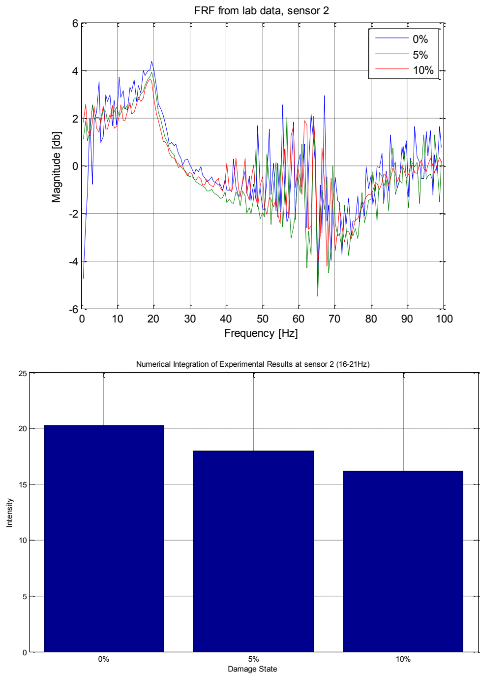
Figure 22: FRF and related bar graph of each damage state for the lab data at sensor 2. There are no 20% or 30% damage states due to the sensor's lead wires becoming detached.
