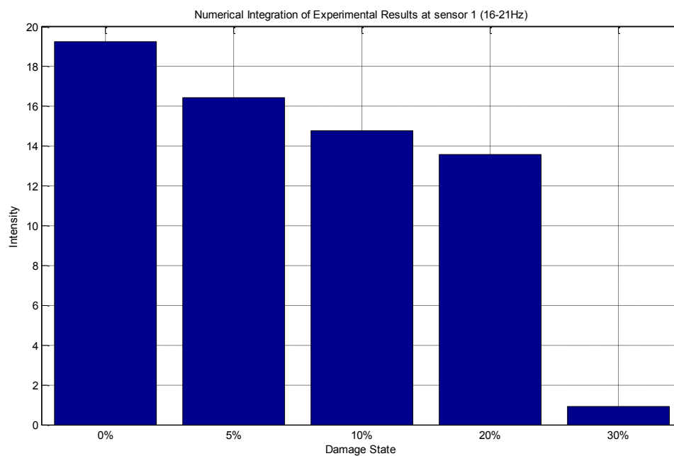
Figure 21: FRF and related bar graph of each damage state for the lab data at sensor 1.
