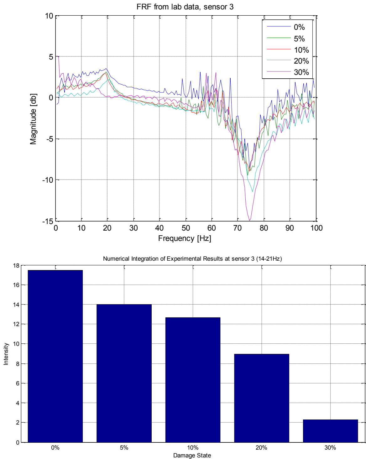
Figure 23: FRF and related bar graph of each damage state for the lab data at sensor 3.
